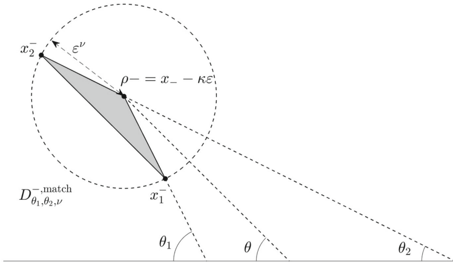
Fig. 6. The matching domain D_{\theta_1, \theta_2, \nu}^{\pm, \text{match}} introduced in (2.32)
